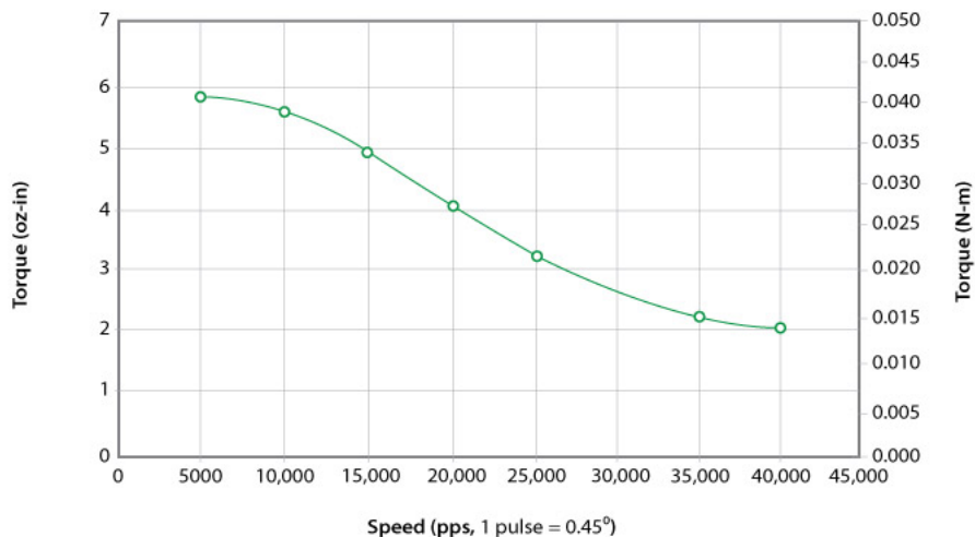
416-07-05 24VDC, 0.6 Amps/Phase, Bipolar, 1/2 Stepping
