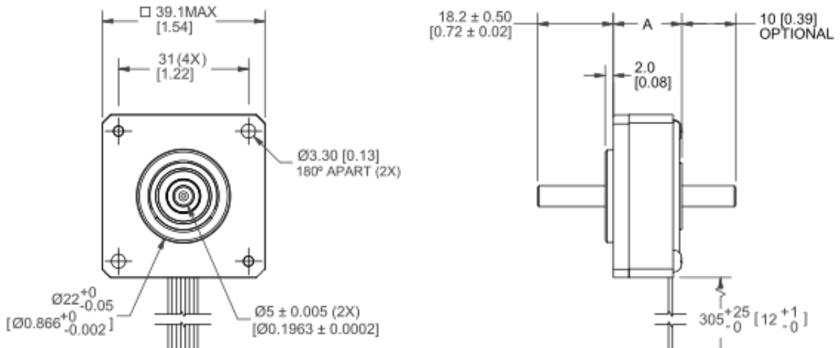
416-07-05 24VDC, 0.6 Amps/Phase, Bipolar, 1/2 Stepping
